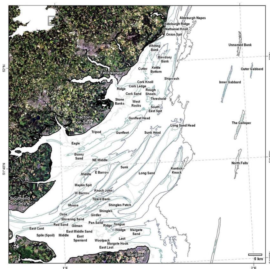
Plate 1.1-3535 The Greater Thames Estuary, showing the main bank features (Burningham; French, 2009).
