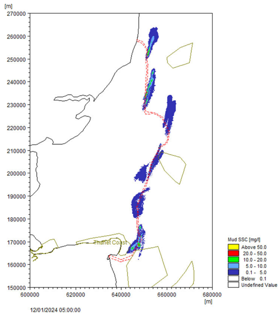
Plate 1.1_3837 Mud SSC levels for jetting installation commencing on spring tides with output on flood (left) and ebb (right) tide after first 24 hours of activity
