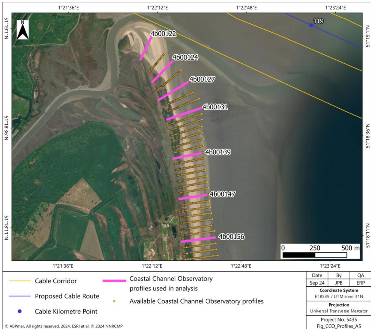
Plate 1.1-2323 Location of topographic profiles available (in yellow) and selected for analysis (in pink) (ABPmer, 2024b).
