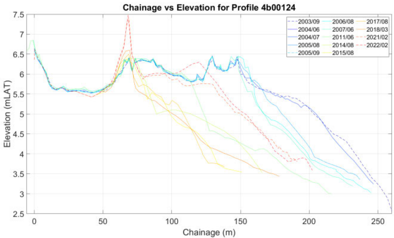
Plate 1.1-2424. Profile 4b000124 elevation change (ABPmer, 2024b)
