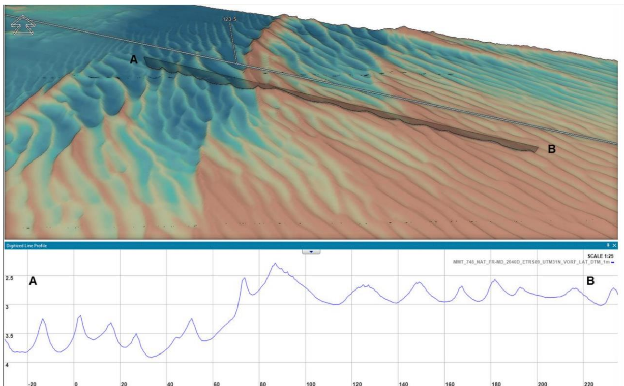
Plate 1.1-2727 Bedforms along the route associated with lee slopes of a mega ripple area at KP 123.475 (MMT, 2022).
