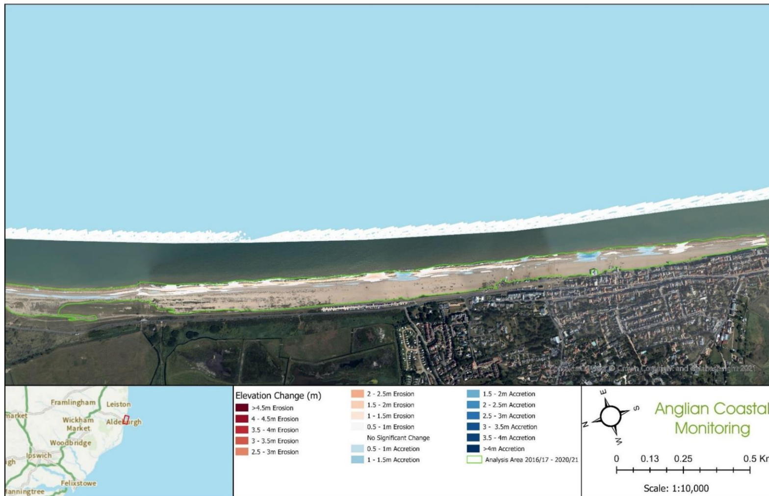
Plate 1.1-1414 The difference in elevation from the LiDAR survey in 2016 and the most recent survey in 2021 for the Aldeburgh monitoring cell (Anglian Regional Coastal Monitoring Programme, 2022).
