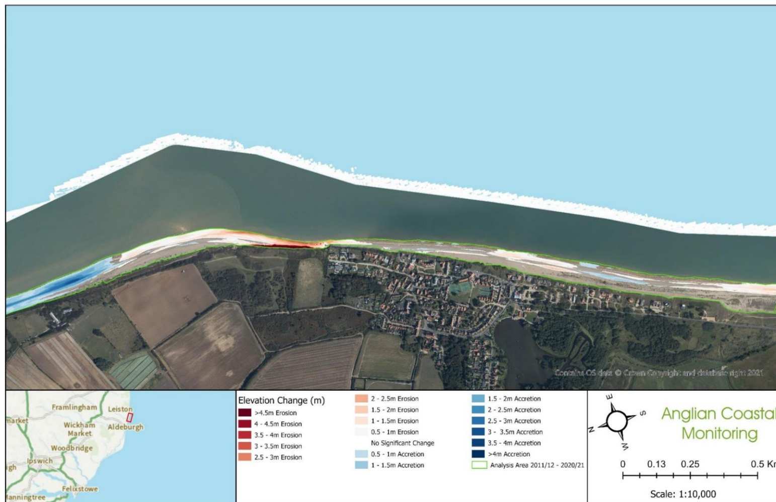
Plate 1.1-1010 The difference in elevation from the first LiDAR survey in 2011 and the most recent survey in 2021 for the Thorpeness monitoring cell (Anglian Regional Coastal Monitoring Programme, 2022).
