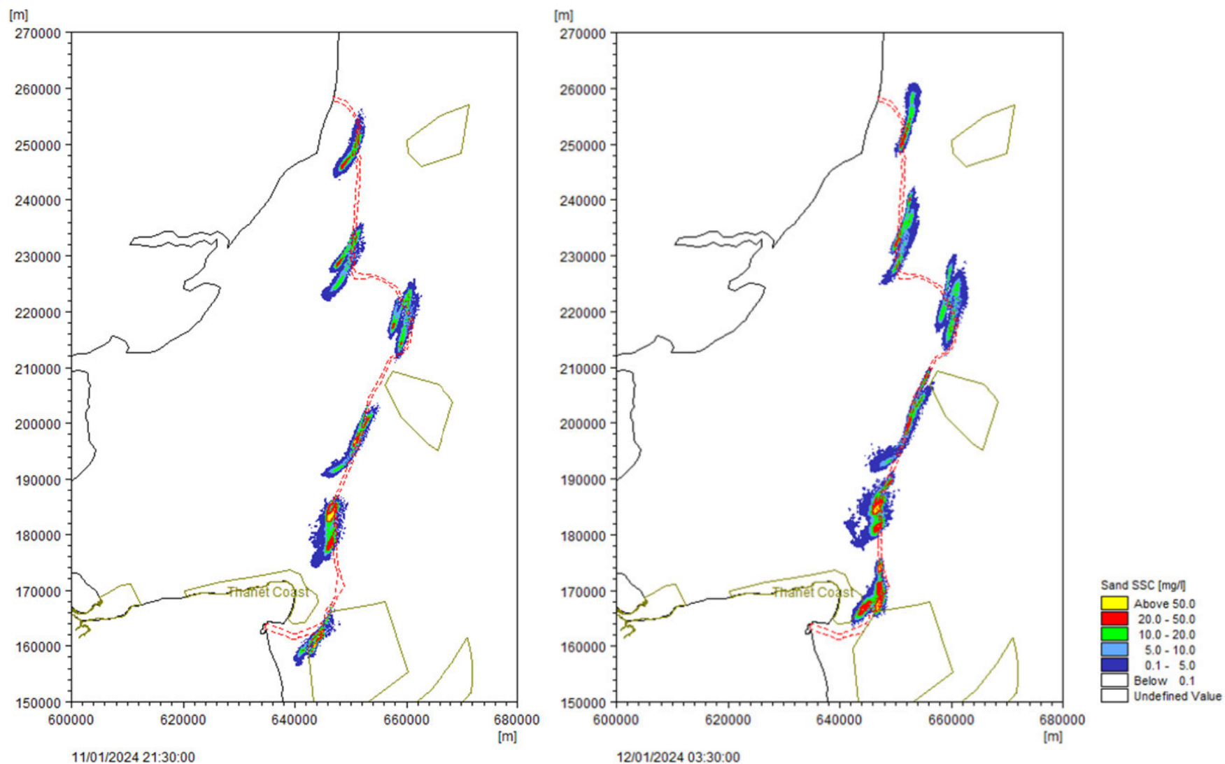
Plate 1.1-4039 Sand SSC levels for jetting installation commencing on spring tides with output on flood (left) and ebb (right) tide after first 24 hours of activity
