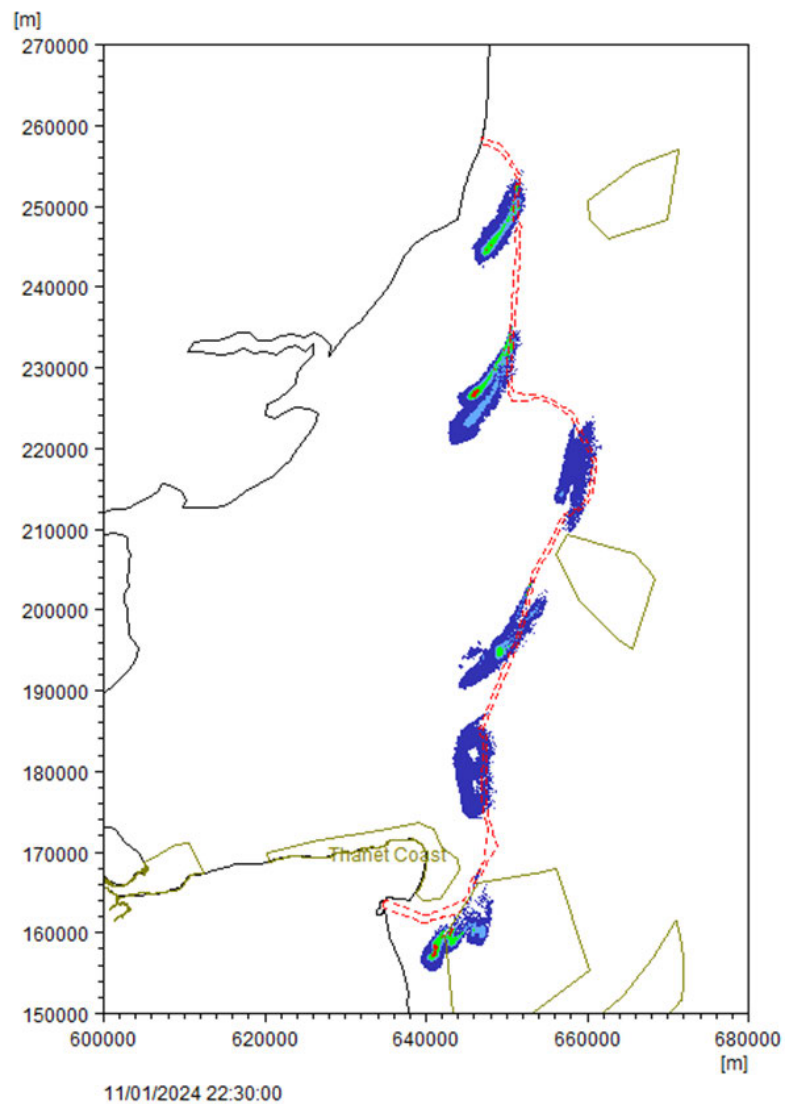
Plate 1.1_3837 Mud SSC levels for jetting installation commencing on spring tides with output on flood (left) and ebb (right) tide after first 24 hours of activity
