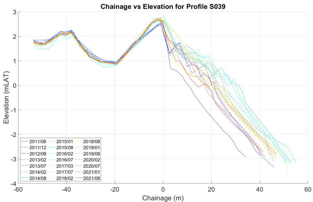
Plate 1.1_1616 Profile changes 2011-2021 – Profile S039 (ABPmer, 2024a)
