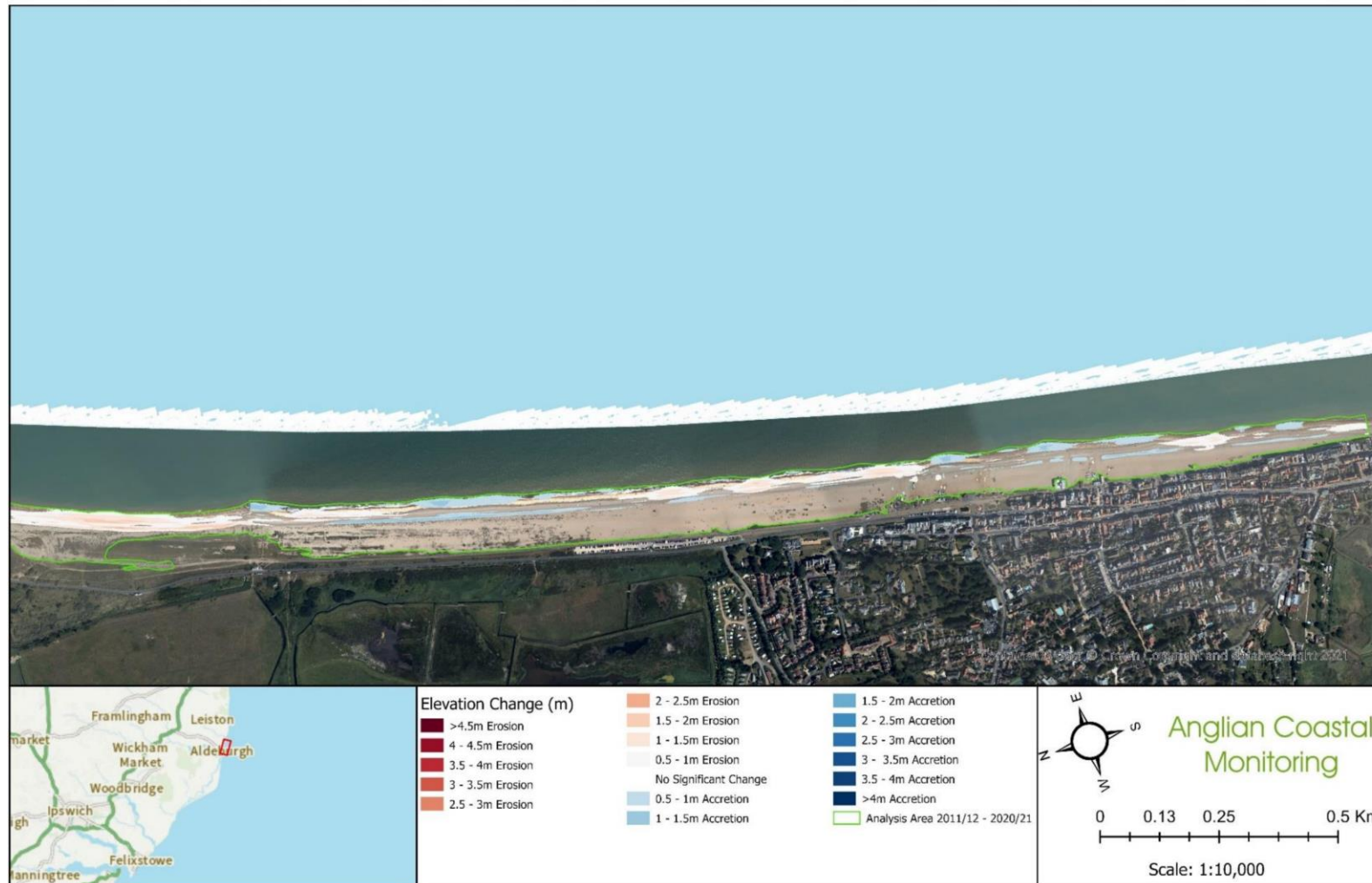
Plate 1.1_1313 The difference in elevation from the LiDAR surveys in 2011 and 2021 for the Aldeburgh monitoring cell (Anglian Regional Coastal Monitoring Programme, 2022).
