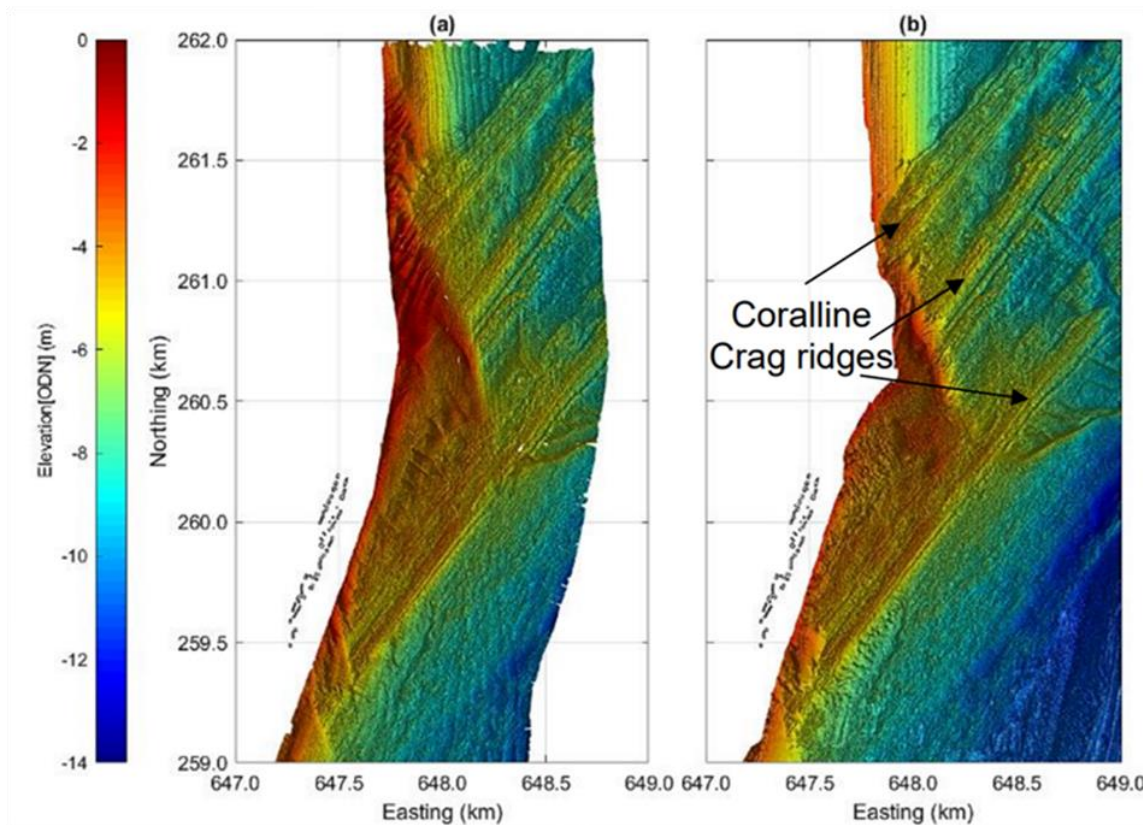
Plate 1.1_55 Bathymetry obtained from two multibeam surveys undertaken by (A) the EA in June 2014 and (B) the Maritime Coastal Authority in January 2017. From (Royal Haskoning DHV, 2019).
