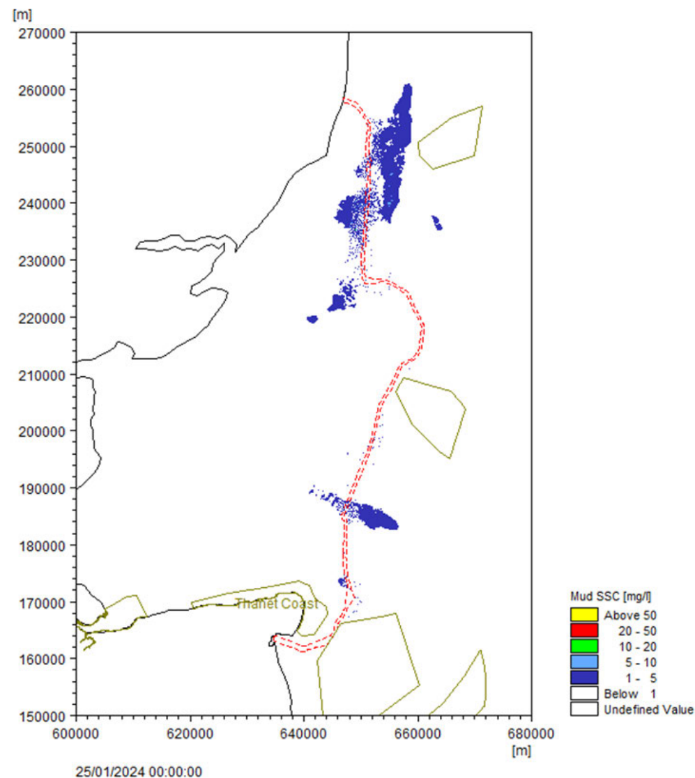
Plate 1.1_3938 Mud SSC levels for jetting installation commencing on spring tides with output at +7 days (left) and +14 days (right) after start of activity
