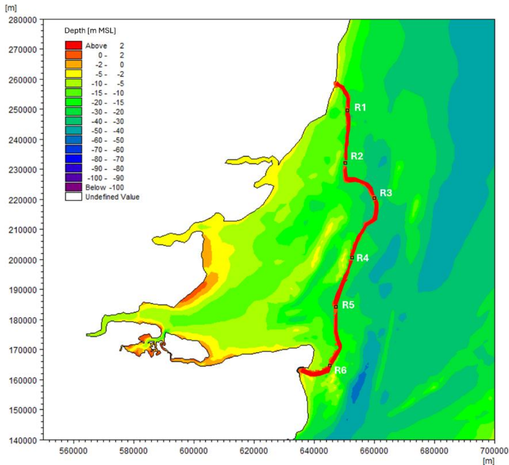
Plate 1.1_3736 Hydrodynamic model bathymetry showing the Offshore Scheme Boundary (red line) and 6 sediment release locations
