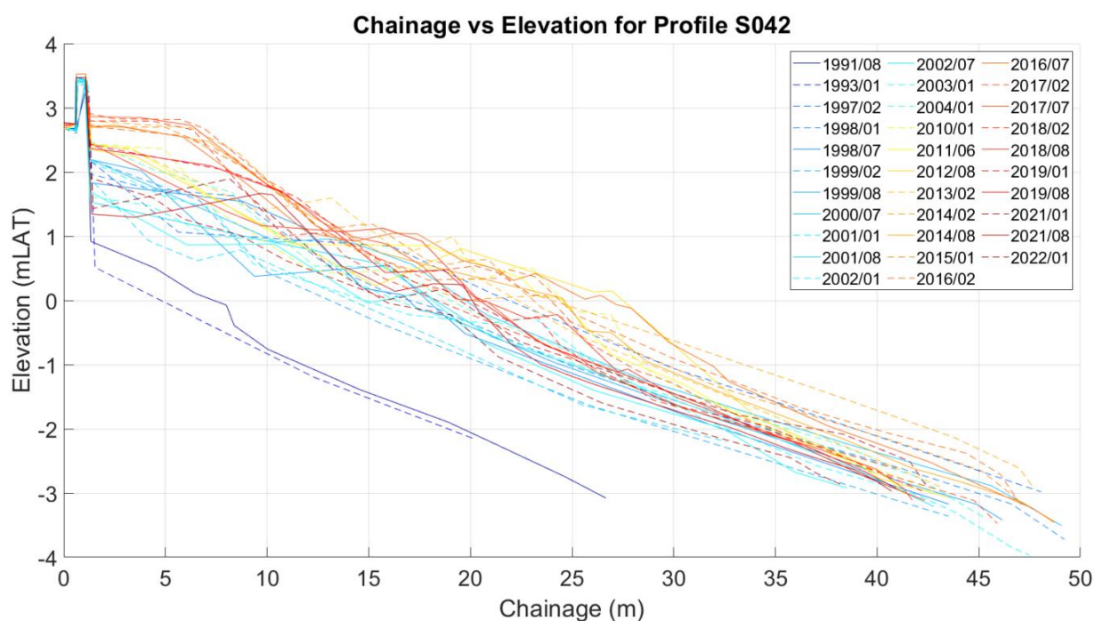
Plate 1.1_1919 Profile changes 2013-2021 – Profile S042 (ABPmer, 2024a)
