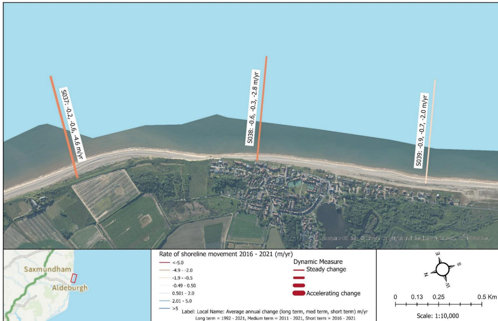
Plate 1.1-1114 Rates of Shoreline Movement (at Mean Sea Level) for the Thorpeness monitoring cell (Anglian Regional Coastal Monitoring Programme, 2022).
